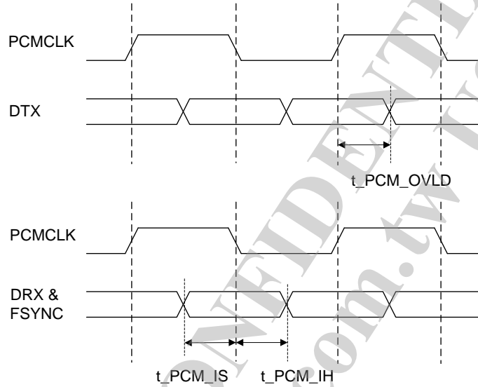
Figure 3-9 PCM Timing
