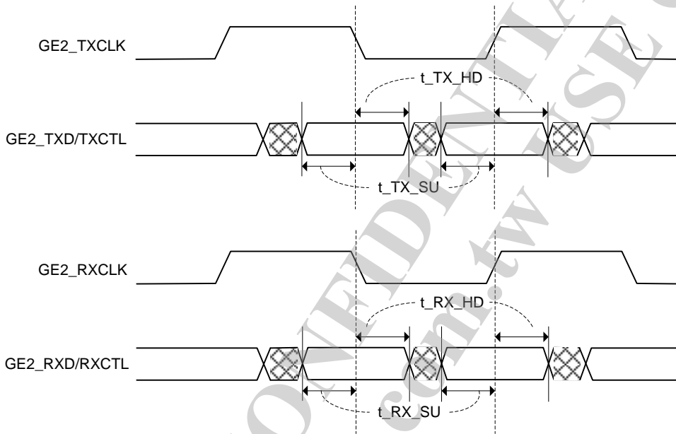
Figure 3-4 RGMII Timing
