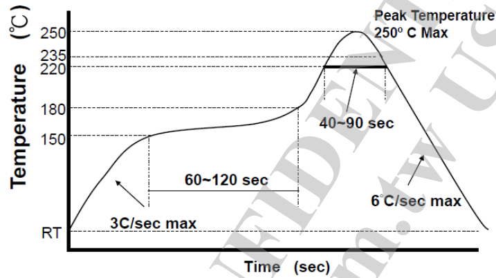
Figure 4-2 Reflow profile
